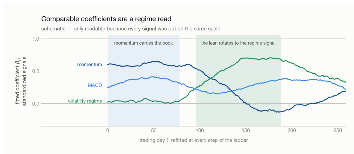
Figure 5.6: Three coefficient paths over a year of refits: momentum decays from high toward zero, a volatility-regime signal rises from zero to become the largest, and MACD stays between them. The shaded stretches mark where momentum carries the book and where the lean rotates to the regime signal.
