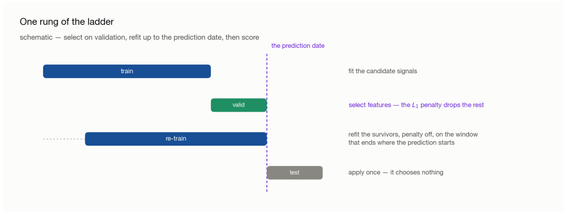
Figure 5.3: One iteration, in four stages: fit on train; select features on the validation segment; refit the survivors on a window shifted forward so that it ends where the prediction starts; apply once to test, beyond the dashed prediction date.
