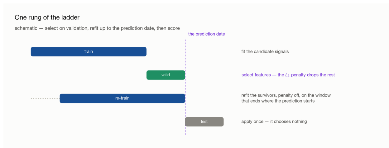
Figure 2: One iteration, in four stages: fit on train; select features on the validation segment; refit the survivors on a window shifted forward so that it ends where the prediction starts; apply once to test, beyond the dashed prediction date.
