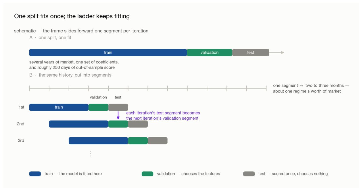
Figure 1: One split against the walk-forward ladder. Above, a single timeline cut once into train, validation and test. Below, the same history divided into twelve equal segments, with the train–validation–test frame starting one segment later on each row—so each row’s test segment is the next row’s validation segment.
