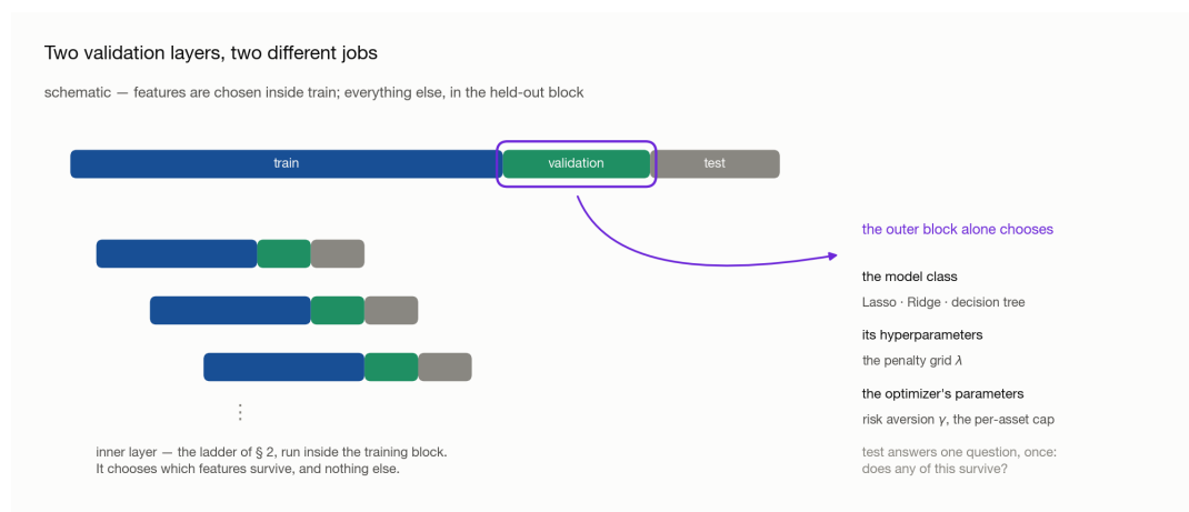
Figure 5.3: The two layers. The inner layer is the miniature ladder inside the training block, which chooses which features survive; the outer layer is the ringed held-out validation block, which chooses the model class, its hyperparameters, and the optimizer's parameters.
