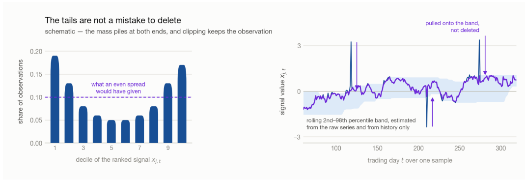
Figure 5.4: Left, the share of observations by decile of the ranked signal—high at the first and last deciles, low in the middle, against the dashed line at 0.1 that an even spread would give. Right, a signal series against a shaded rolling percentile band, with the spikes that reach outside it pulled back onto its edge.
