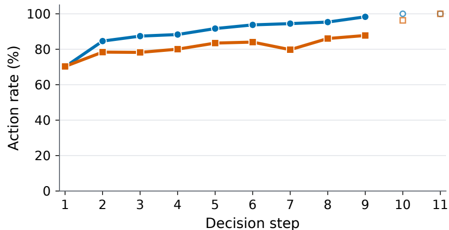
Action keeps goal reachable
