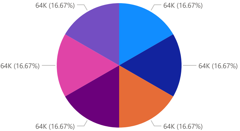
Sum of quantity_kg by sku_id
