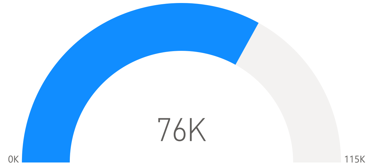
used_capacity_kg and capacity_kg
