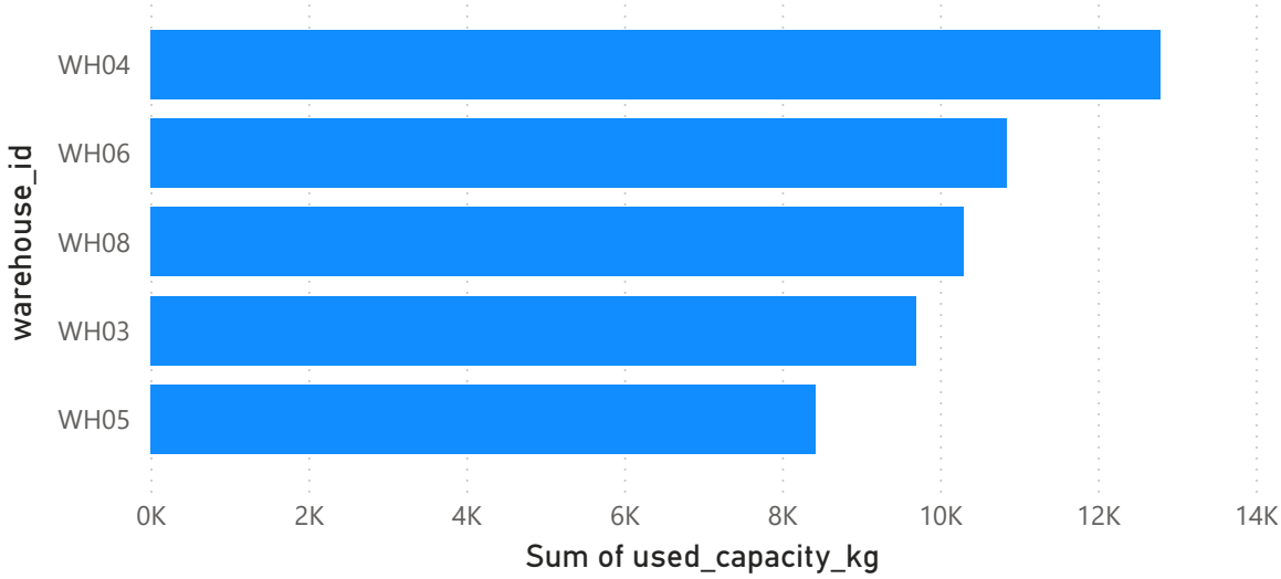
Sum of used_capacity_kg by warehouse_id
