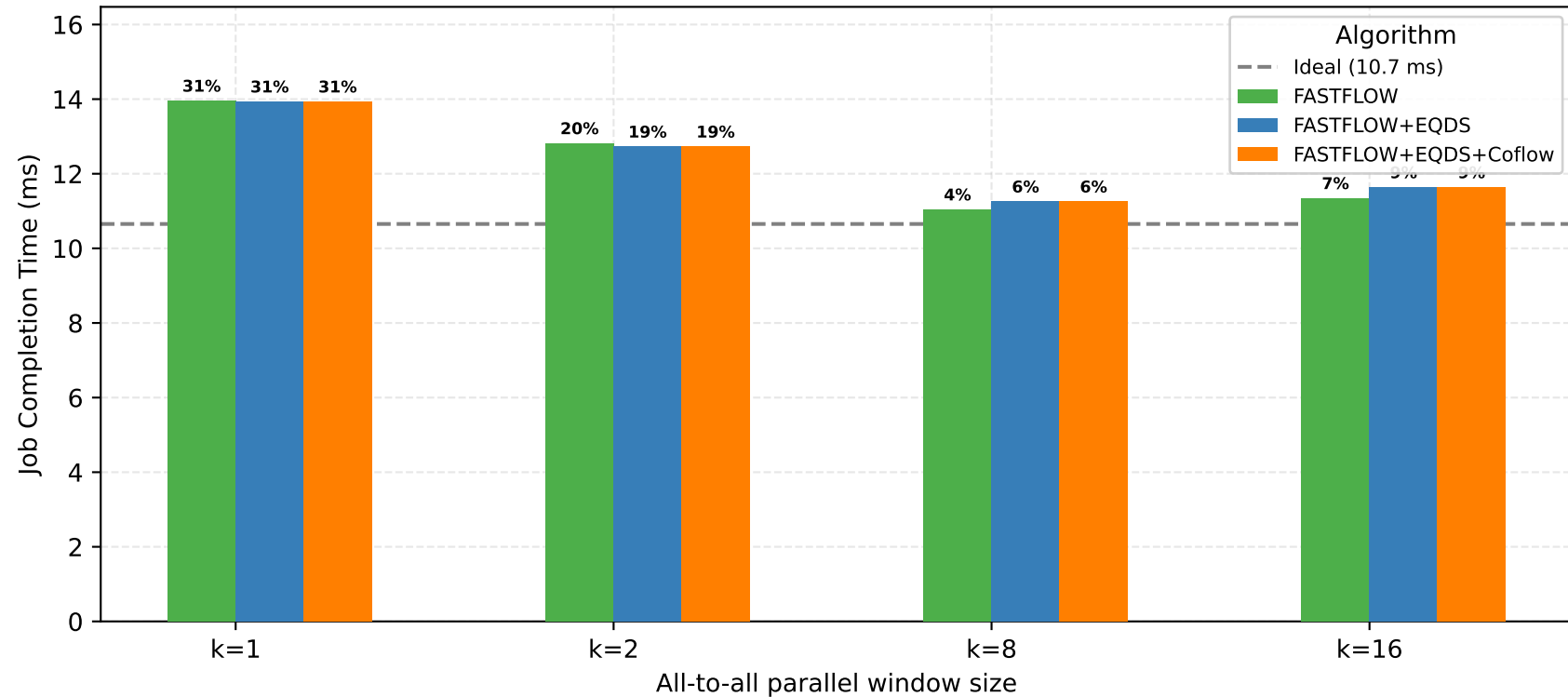
Performance in several all-to-all scenarios · 1MiB message 128 Nodes · 8:1 OS · 800Gbps · 4KiB MTU
