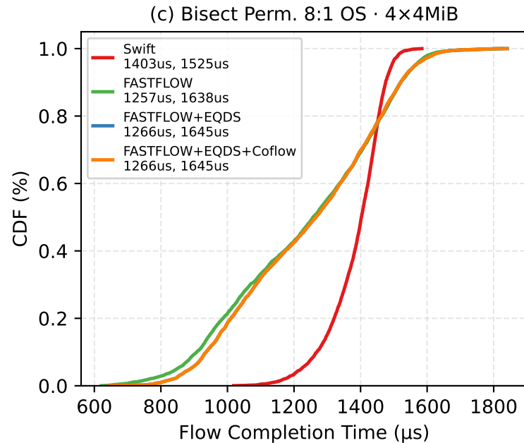
Flow completion time for different permutations on fat trees with different oversubscription ratios.
