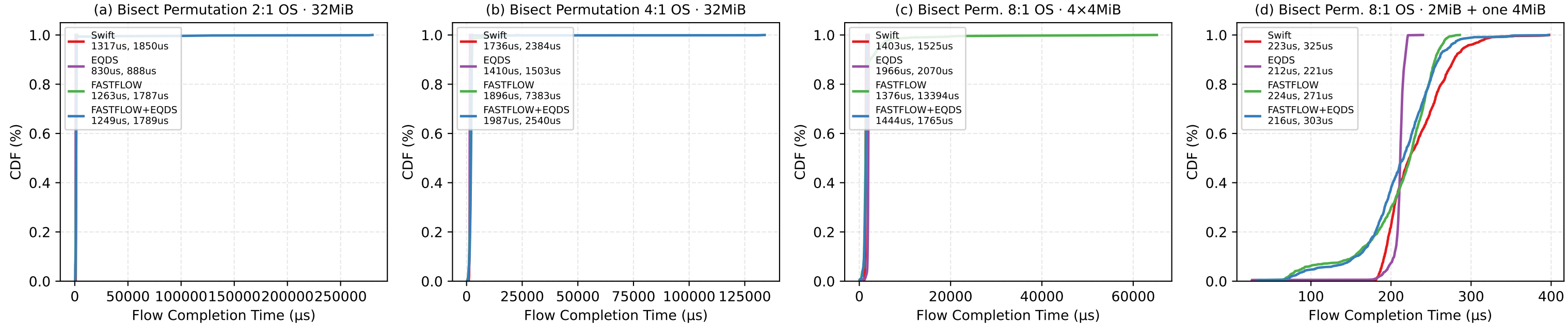
Flow completion time for different permutations on fat trees with different oversubscription ratios.
