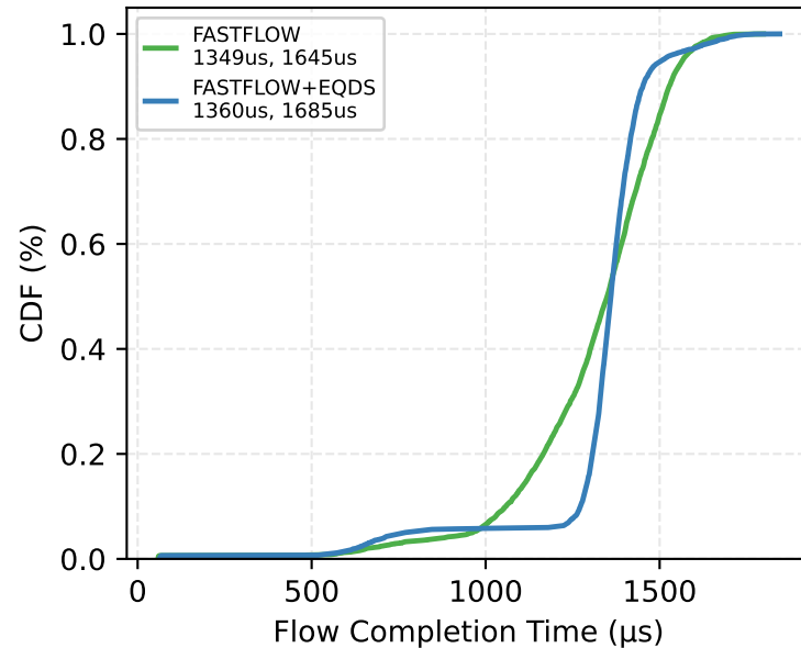
(c) Bisect Perm. 8:1 OS · 4×4MiB
