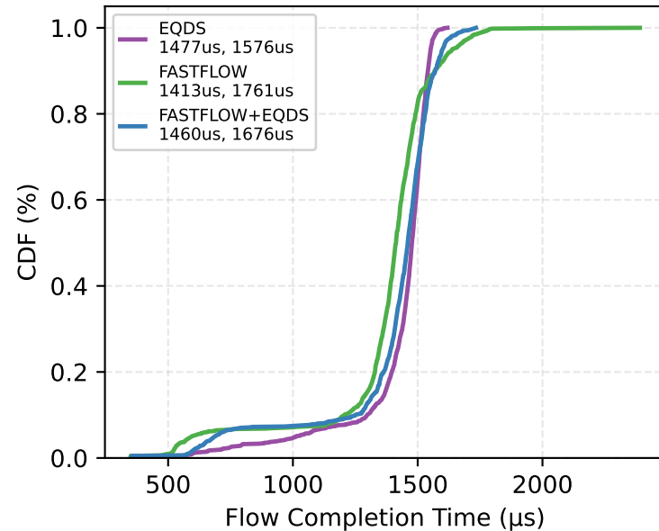
(b) Bisect Permutation 4:1 OS · 32MiB
