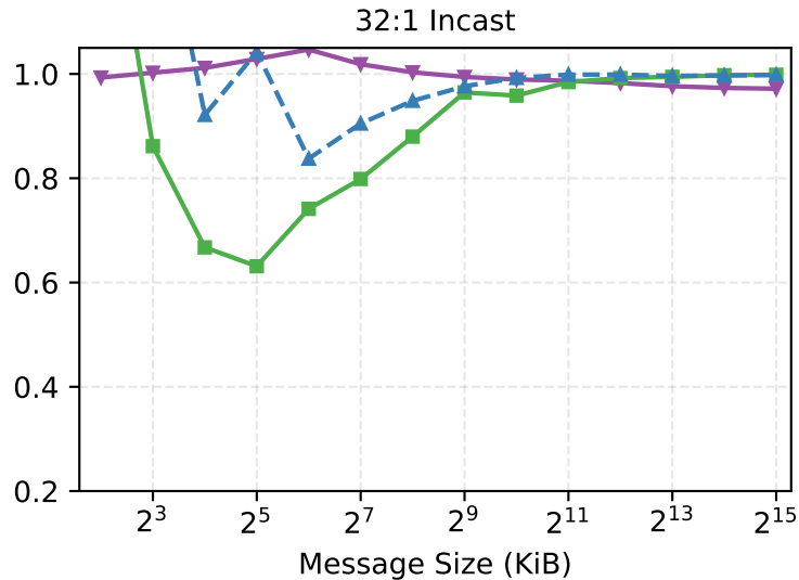
Message Scaling During Incast 1024 Nodes · 800Gbps · 4KiB MTU
