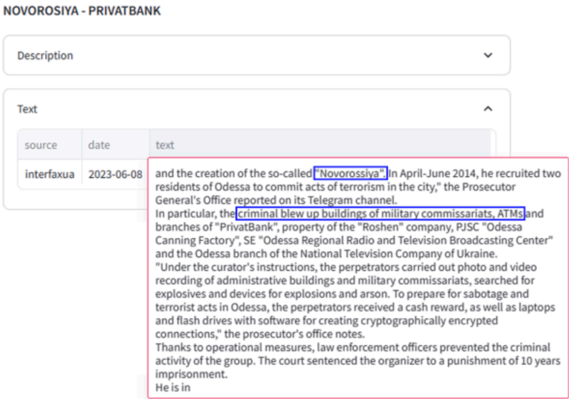
Figure 2: GraphRAG provenance
