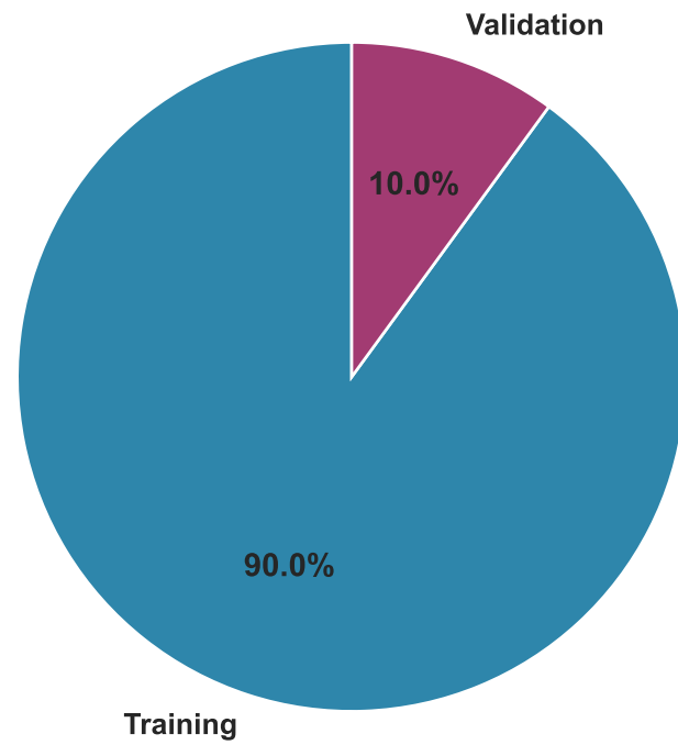
Dataset Split
