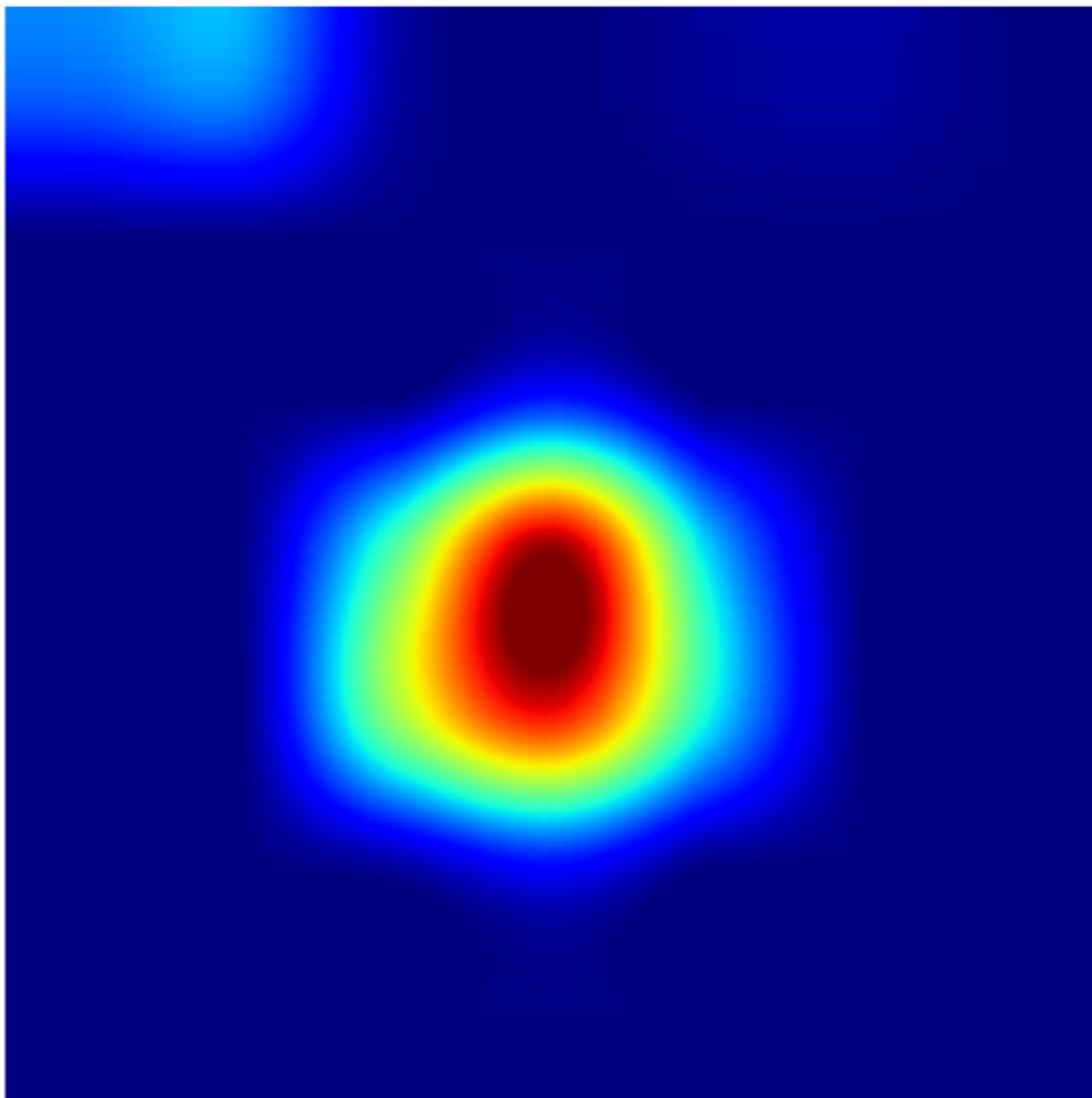
Grad-CAM Heatmap
