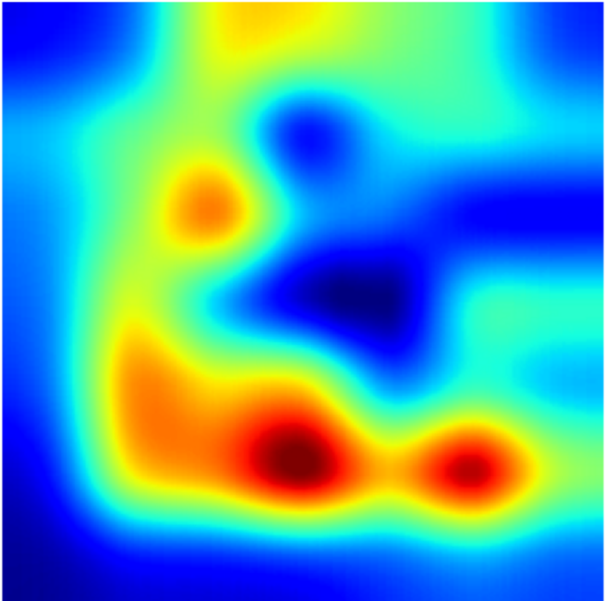
Grad-CAM Heatmap
