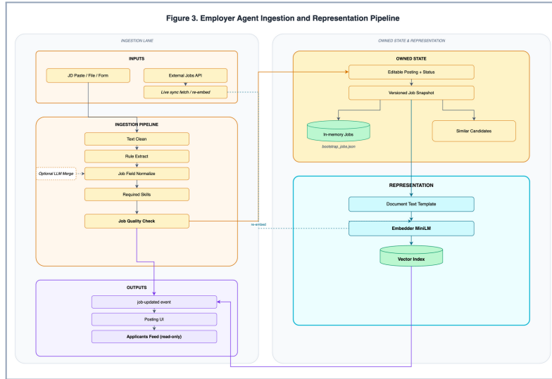
Fig. 3: Internal structure of the Employer agent: JD ingestion (clean, rules, optional LLM), job quality check, posting status lifecycle, optional external feed sync, job snapshots, and side outputs (events, applicants feed, similar candidates).
