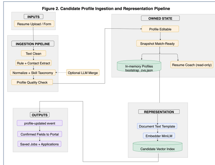
Fig. 2: Internal structure of the Candidate/Client agent: document ingestion (clean, rule extract, optional LLM merge), skill normalization, profile quality check, editable profile versus match-ready snapshot, embedding, and side outputs (events, activity store, resume coach).
