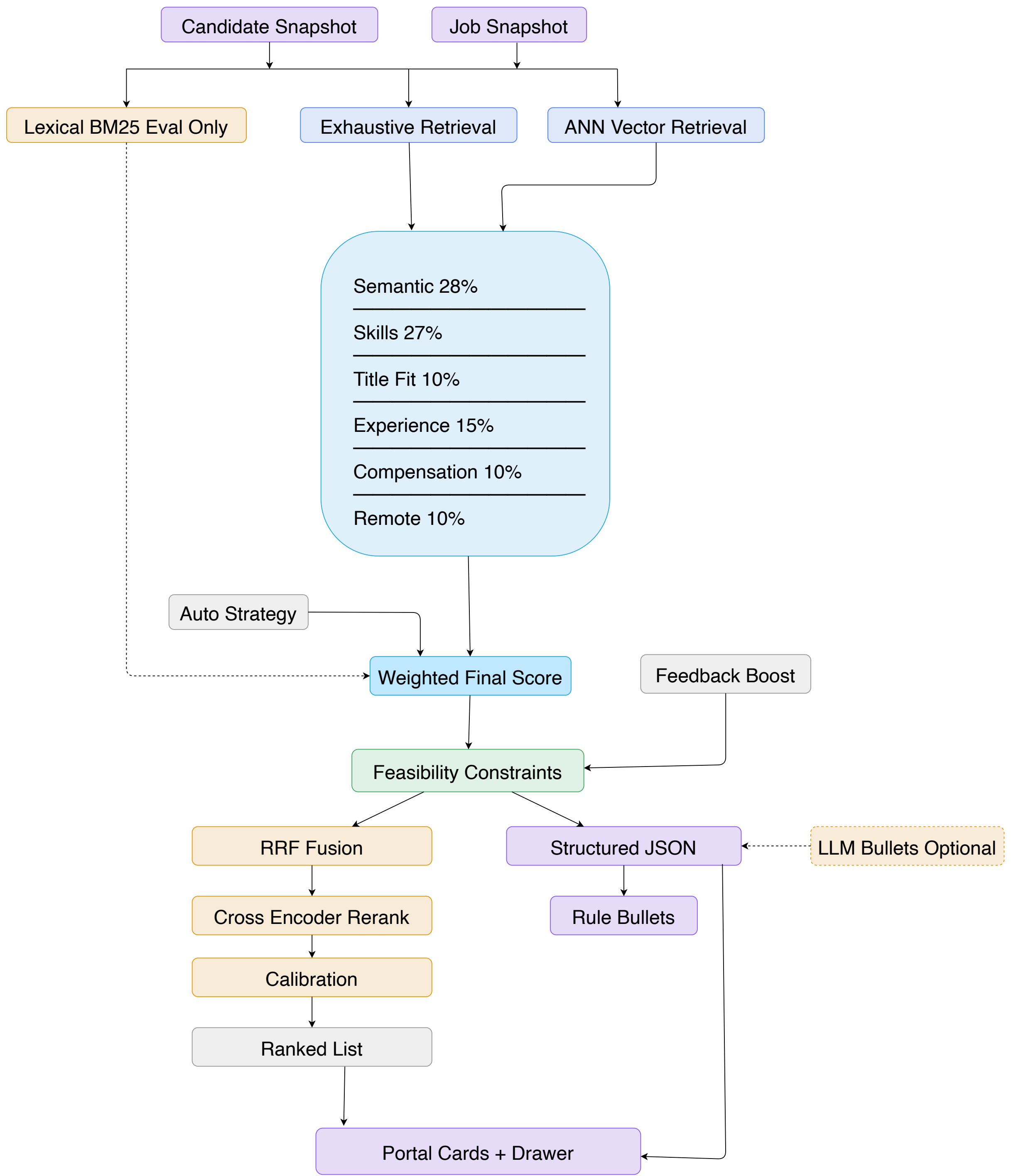
Figure 8. Matching, Ranking and Explanation Pipeline
