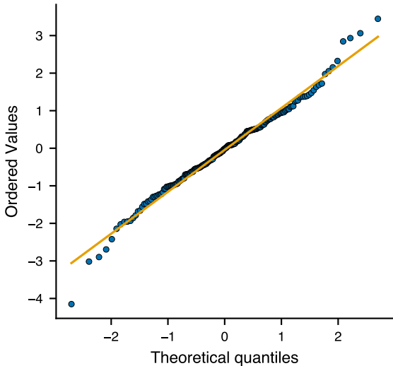
Q-Q plot (normality)
