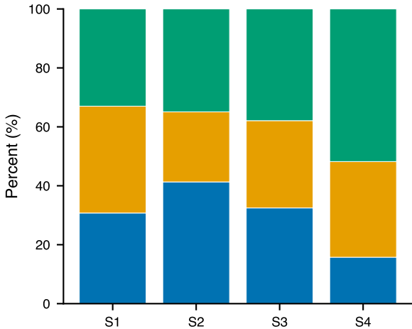
100% stacked bar
