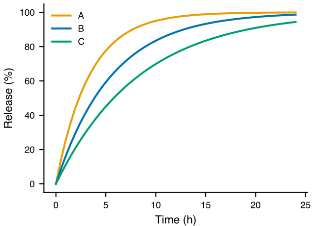
Multi-series line
