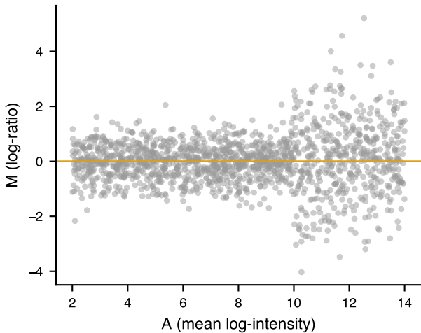
MA plot
