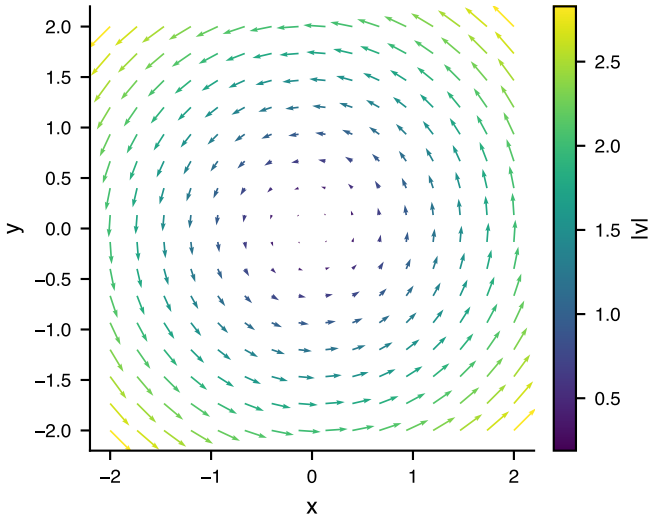
Quiver (vector field)
