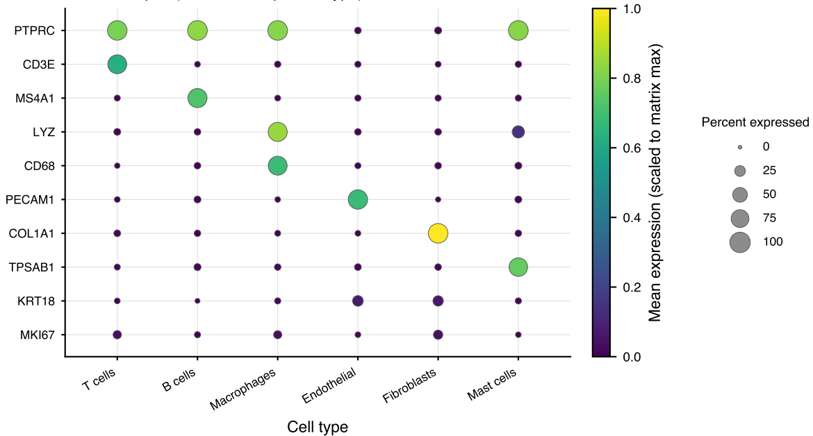
Marker dot plot (n = 220 cells per cell type)
