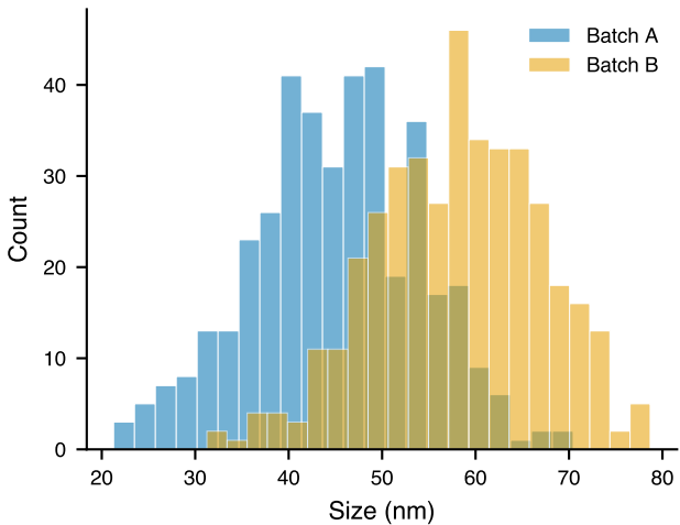
Overlaid histograms
