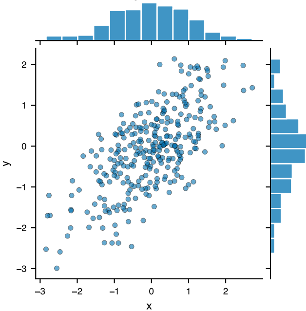
Scatter + marginals
