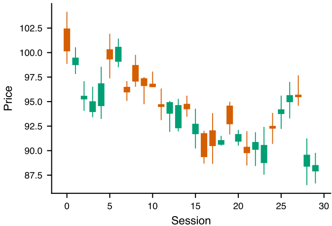
Candlestick (OHLC)
