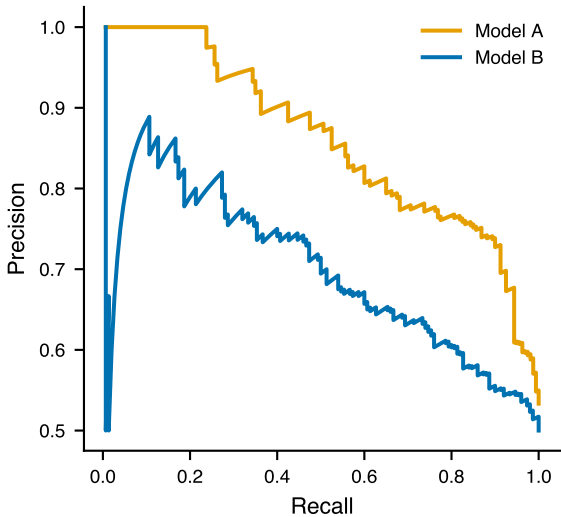
Precision–recall
