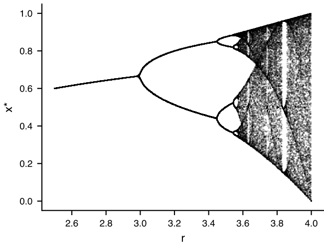
Bifurcation diagram
