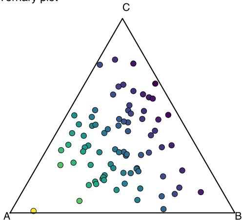
Ternary plot
