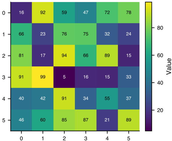
Annotated heatmap
