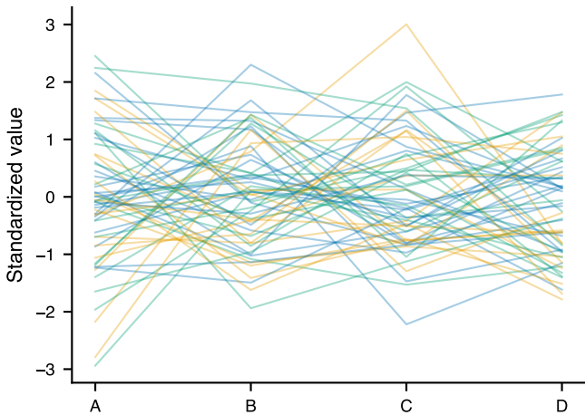
Parallel coordinates
