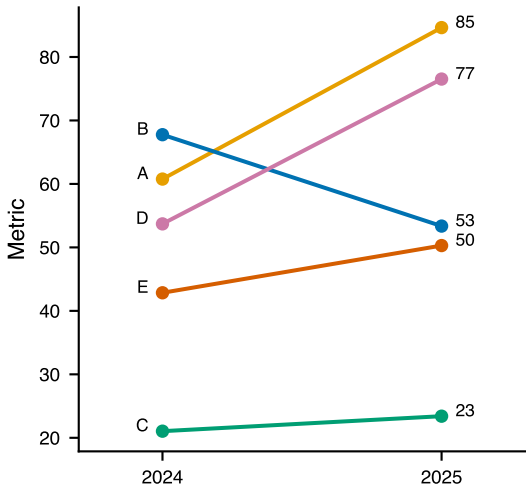
Slope chart
