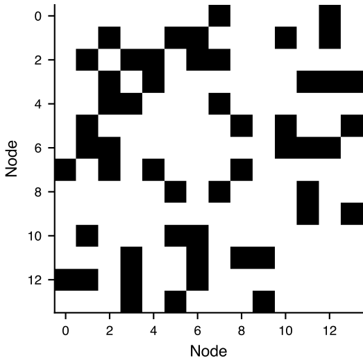
Adjacency matrix
