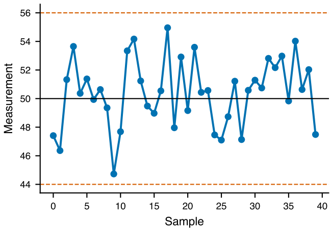
Control chart (SPC)
