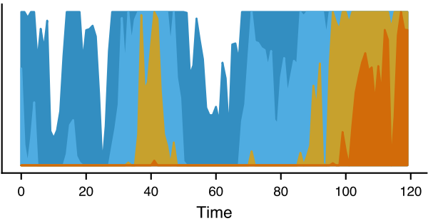
Horizon chart
