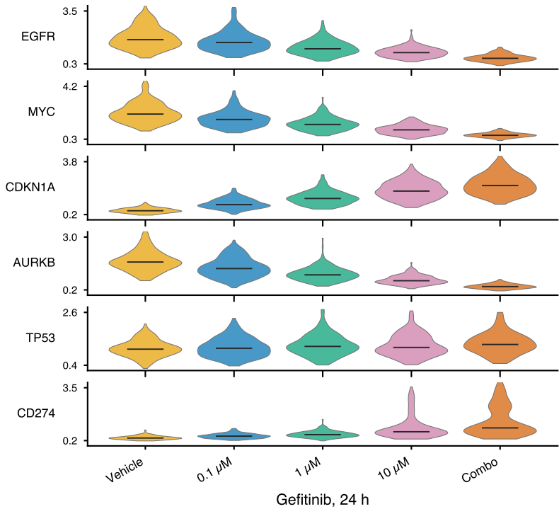
Log-normalised expression, scaled per gene
