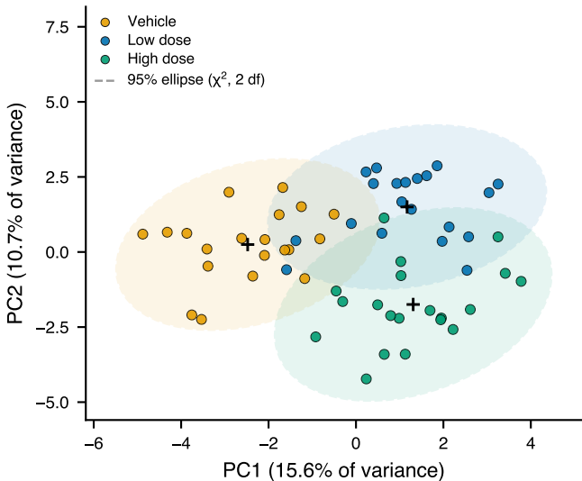
PCA scores + 95% group ellipses (n = 20/group, p = 30)
