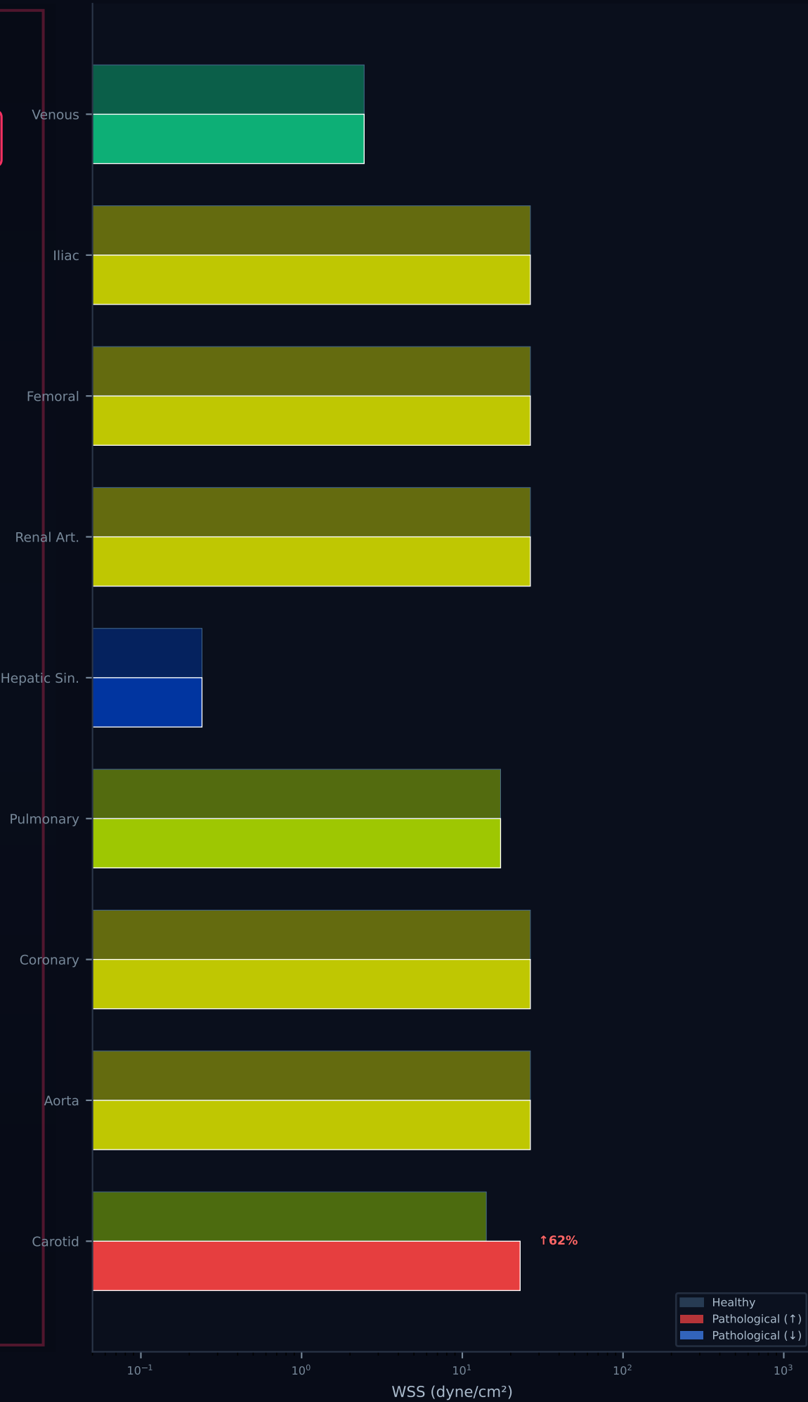
WSS Comparison Healthy vs Brain Tumor (Glioblastoma)
