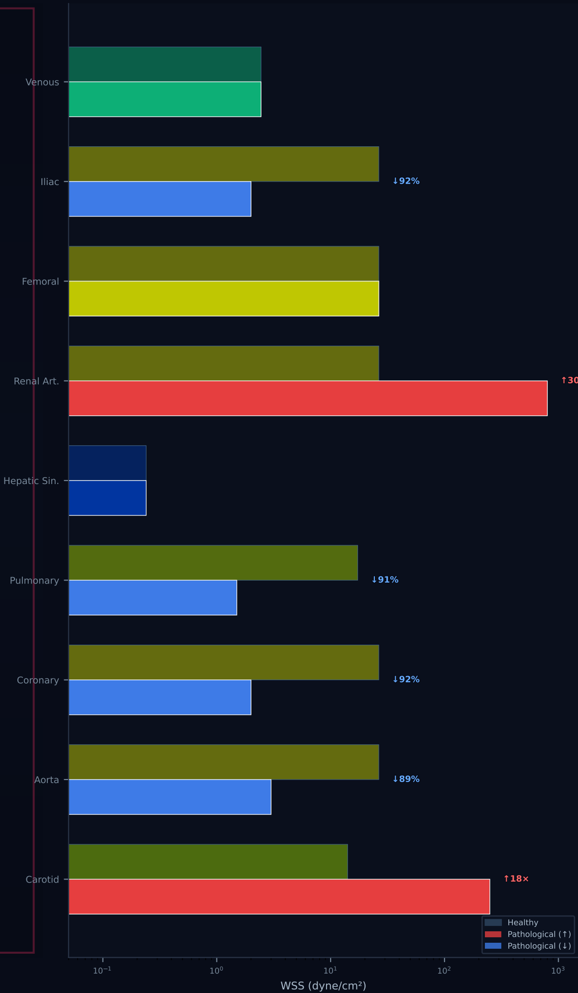
WSS Comparison Healthy vs Combined Severe Pathology
