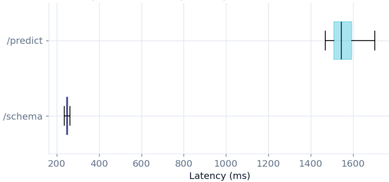
Latency distribution per request
