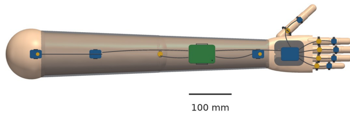
Figure 2. One sleeve per arm. (a) Isometric view. (b) Top view to scale. Blue lids are motion sensors, gold lids are vibration motors, green is the hub.
