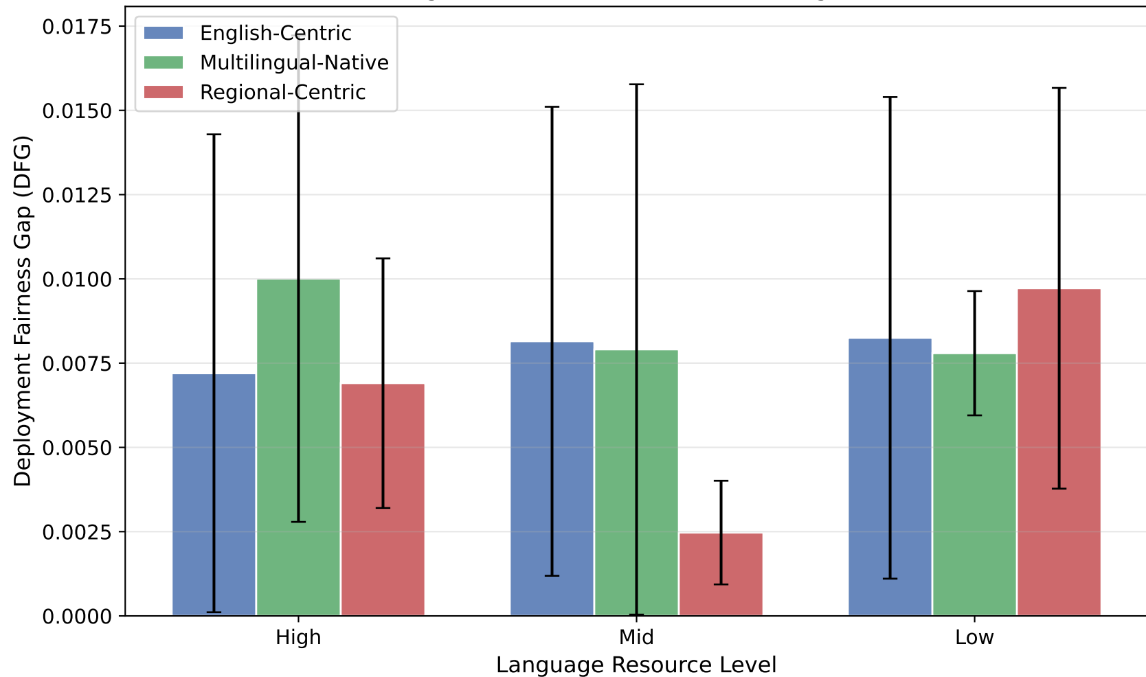
Deployment Fairness Gap by Language Resource Level (higher = less fair treatment vs. English)
