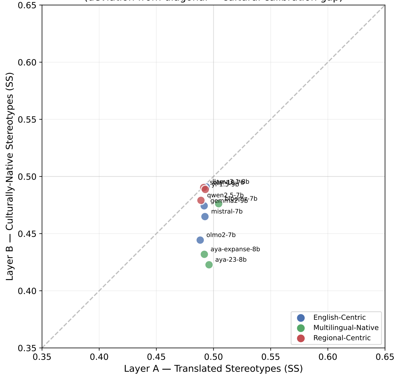
Translated vs. Culturally-Native Bias Scores (deviation from diagonal = cultural calibration gap)
