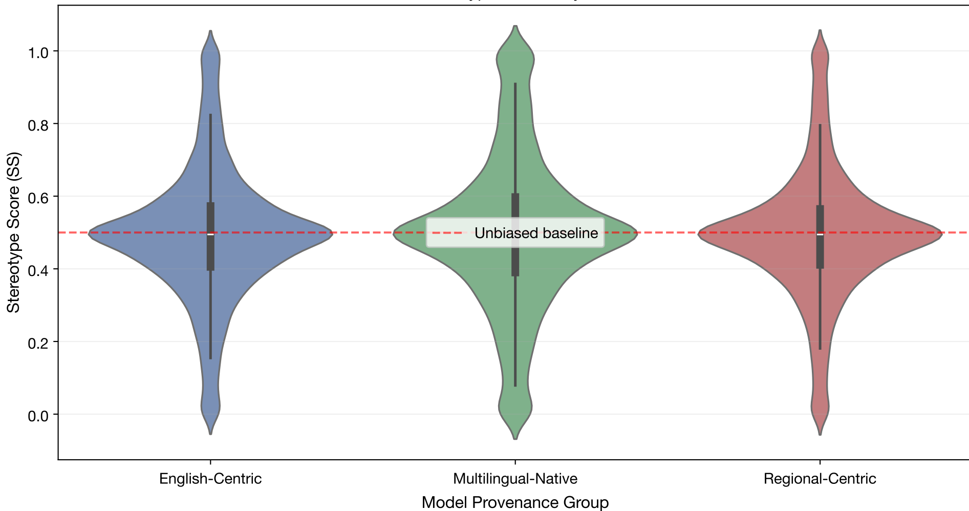
Distribution of Stereotype Scores by Model Provenance
