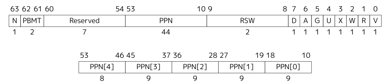
Figure 71. Sv57 page table entry.
