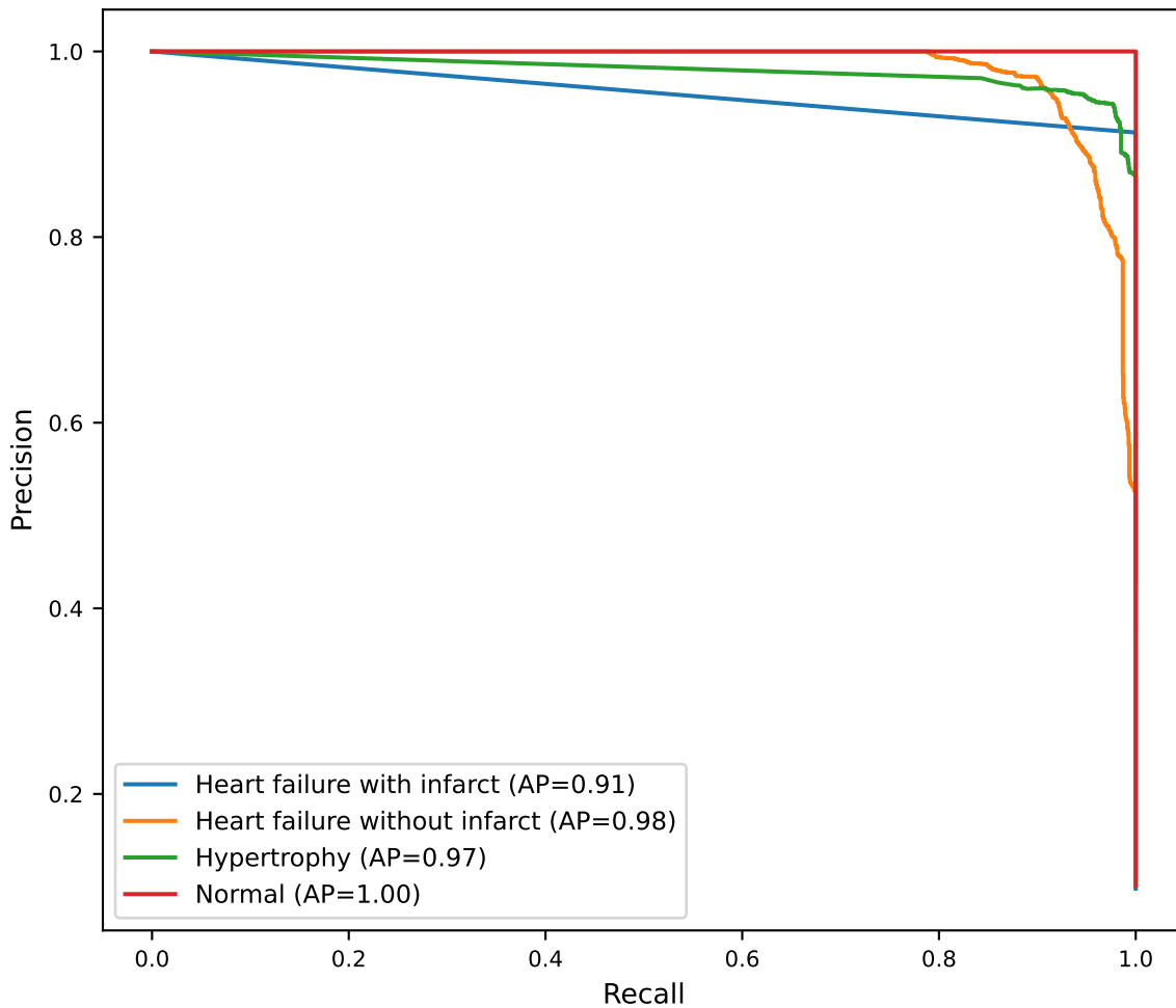
Precision-Recall Curves (Full Dataset)
