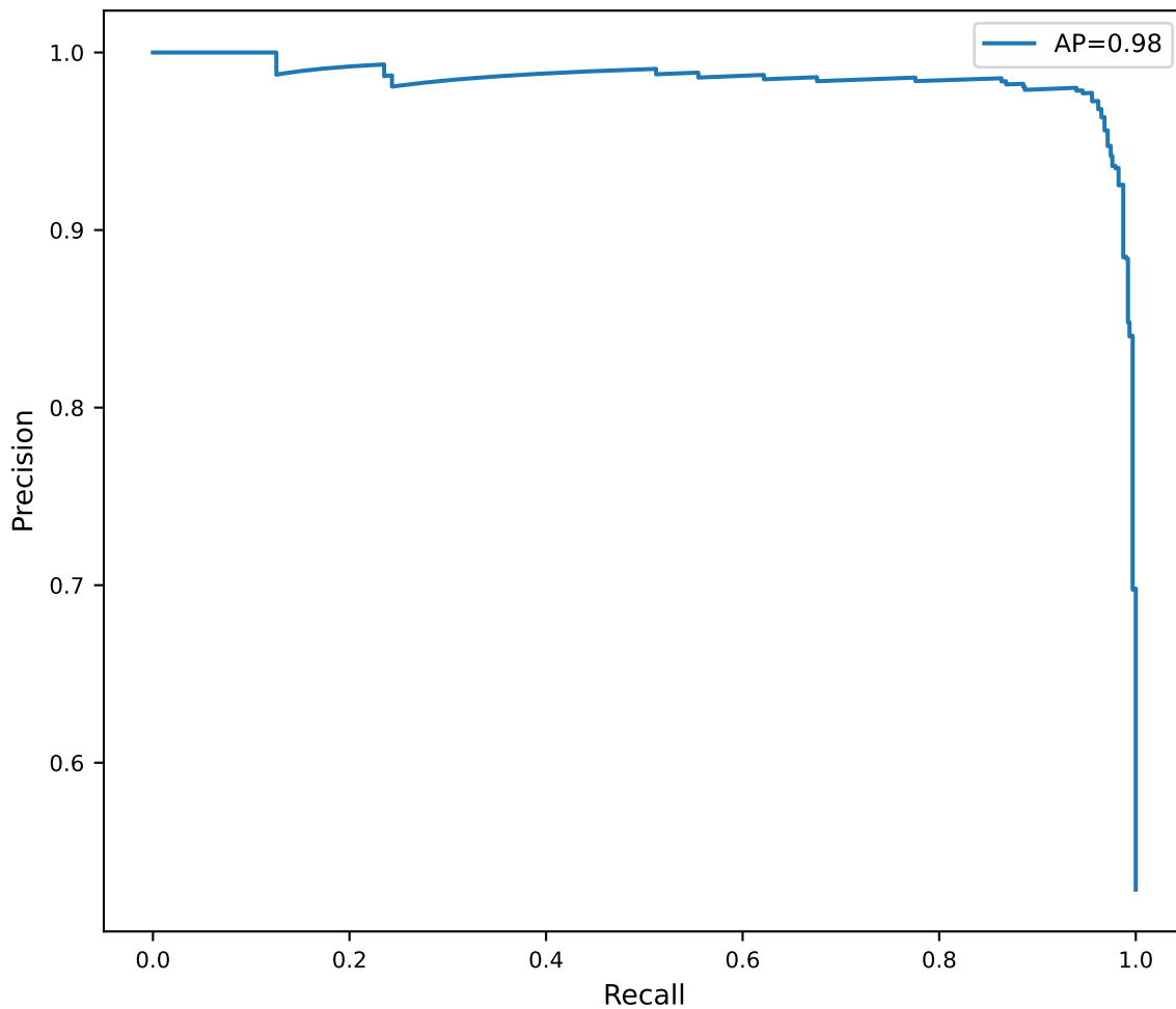
Precision-Recall Curve (Patient-Level)
