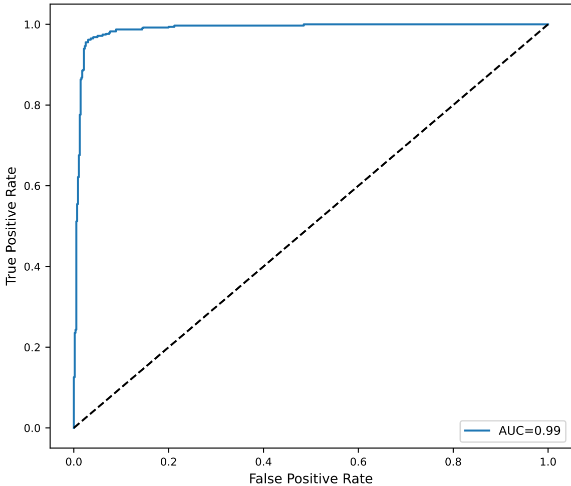
ROC Curve (Patient-Level)
