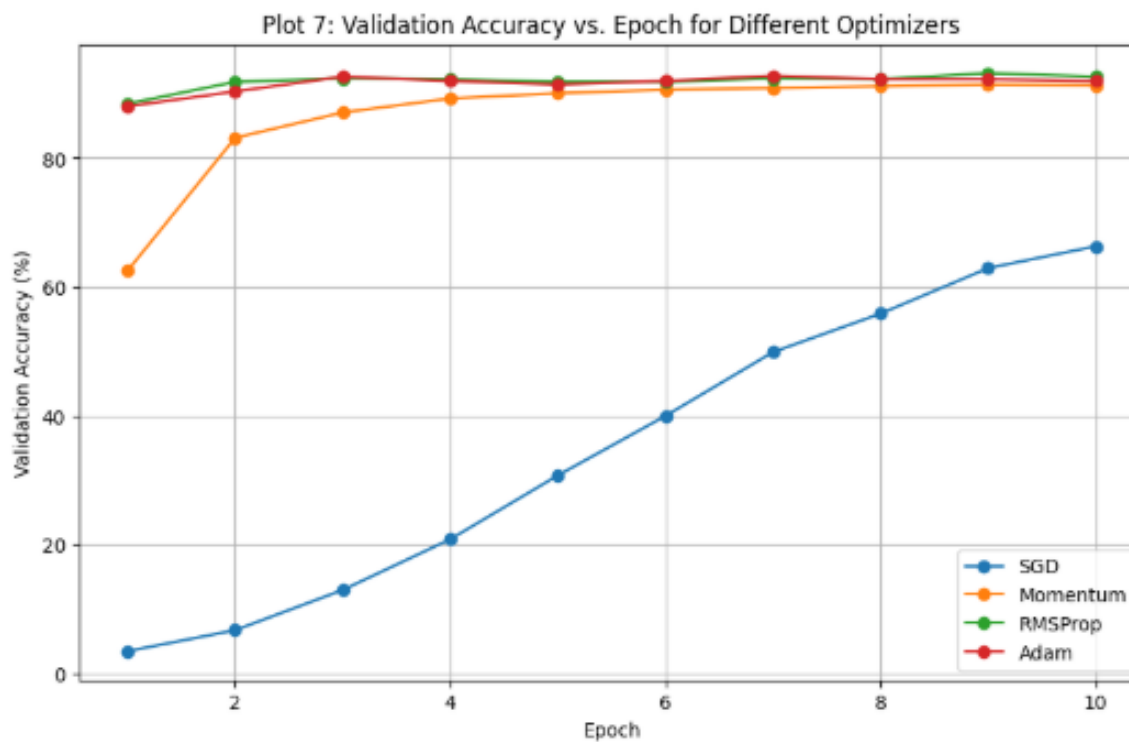
Figure 13: Validation Accuracy vs. Epoch for Different Optimizers
