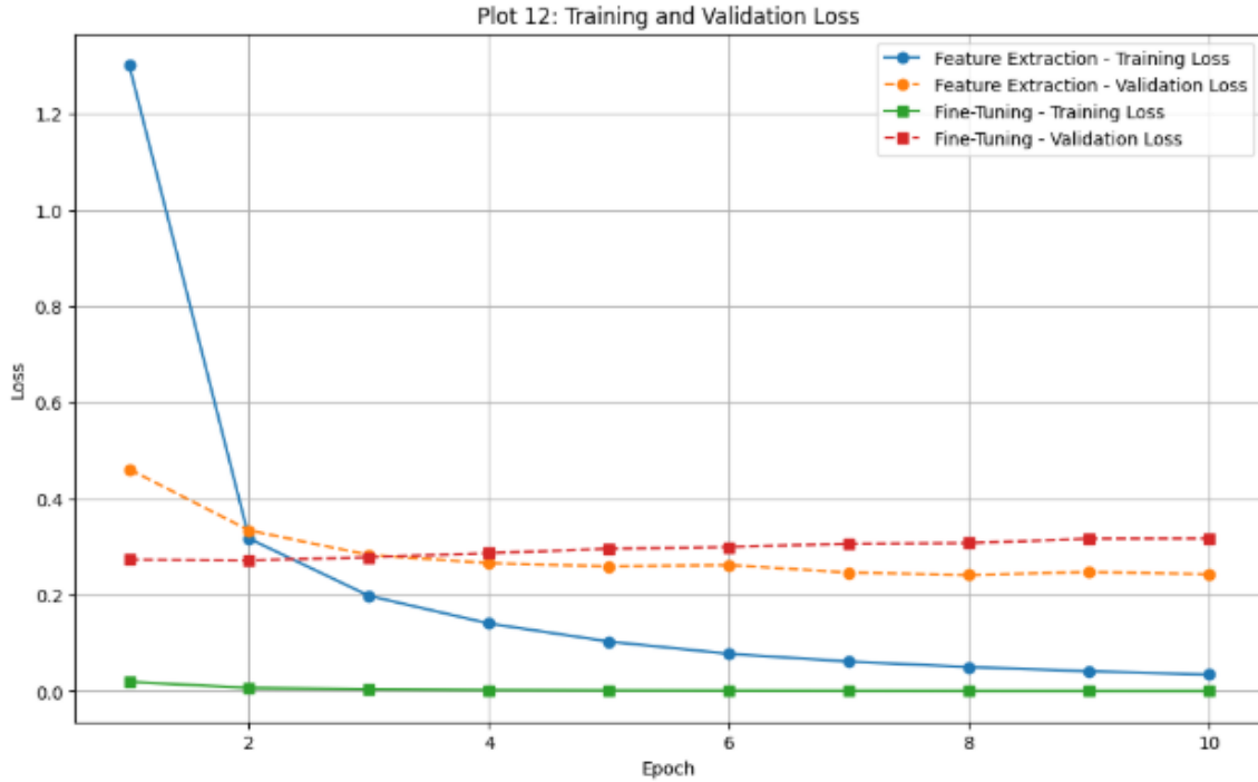
Figure 18: Training and Validation Loss for Feature Extraction and Fine-Tuning
